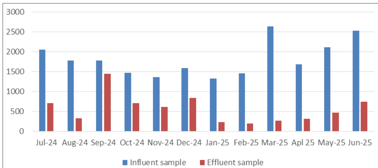
Fig 5: COD (mg/l)
