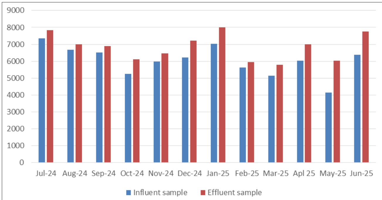
Fig 6: TDS (mg/l)
