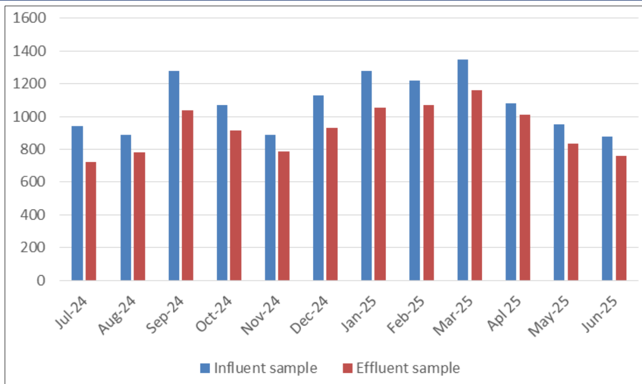
Fig 4: Hardness (mg/l)
