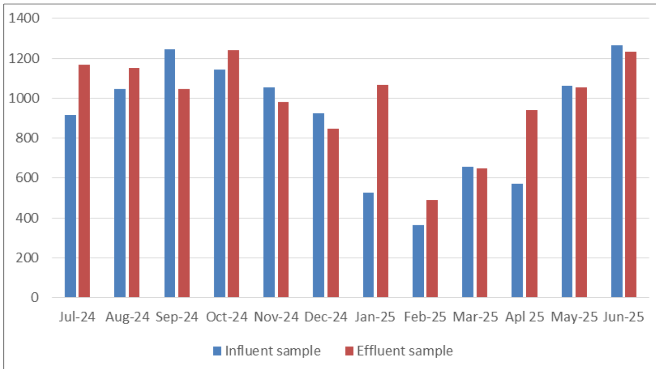
Fig 7: Sulphate (mg/l)
