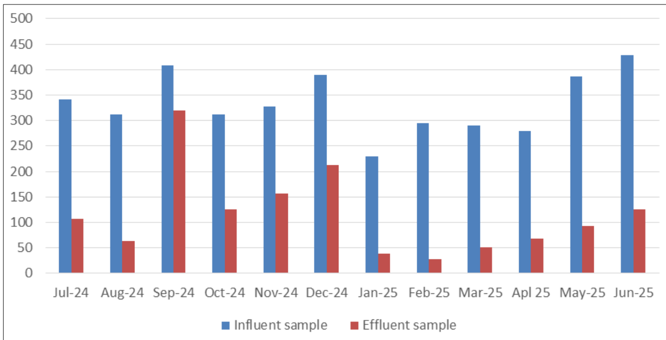
Fig 3: BOD (mg/l)
